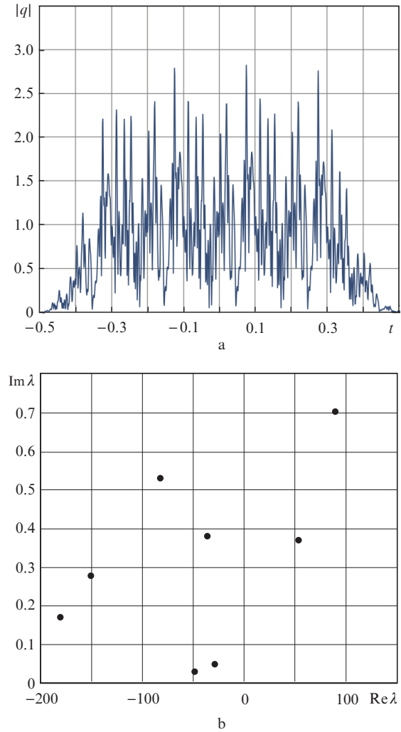
Figure 1. (a) Example of the dependence of the amplitude of the WDM signal under study on time (one of the possible implementations is given), and (b) example of the location of the discrete spectrum components in the complex half-plane of the spectral parameter \lambda for one of the signals under study.
