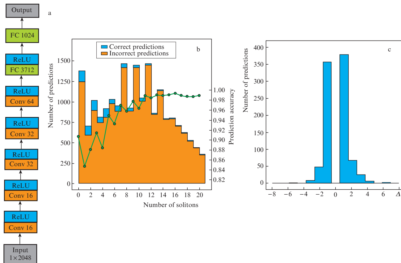
Figure 2. (Colour online) (a) Neural network architecture for predicting the number of discrete eigenvalues (solitons) in the nonlinear Fourier spectrum for a WDM signal [39], (b) the distribution of correct and incorrect predictions of the neural network as a function of the number of solitons in signals from the validation sample (the green curve shows the network prediction accuracy for each set of signals with the same number of solitons), and (c) the distribution of the deviation \Delta of the predicted number of solitons in the signals from the validation sample versus their actual number.
